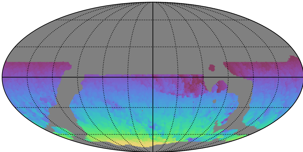
weather_cloudso10v3.4_10yrs WFD all bands: Max HA
