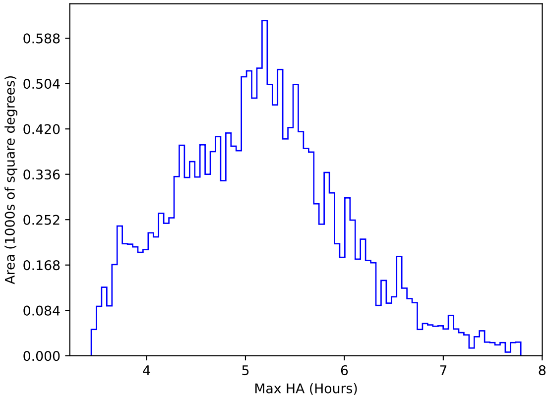
weather_cloudso10v3.4_10yrs WFD all bands: Max HA
