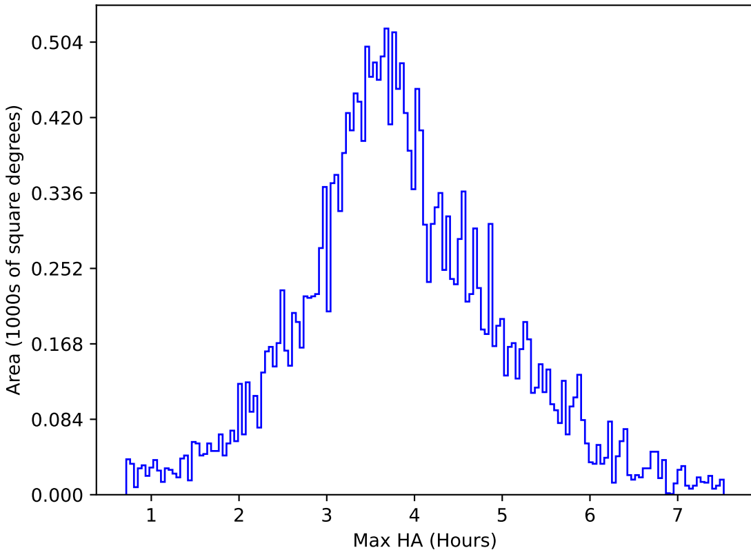
weather_cloudso10v3.4_10yrs All sky u band: Max HA
