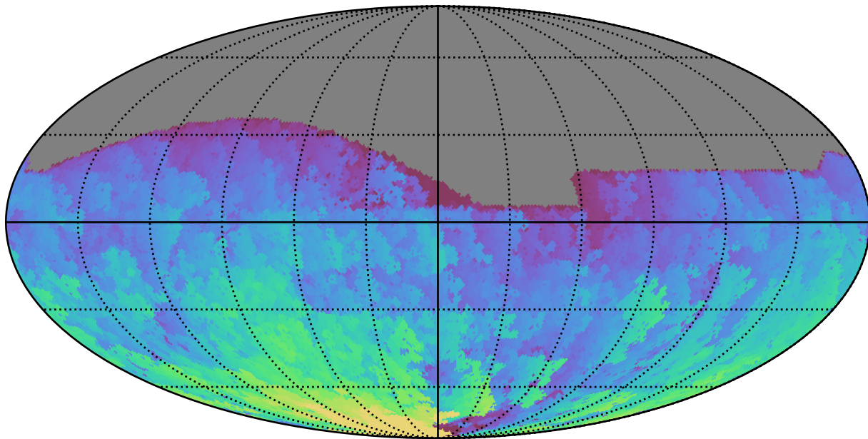
weather_cloudso10v3.4_10yrs All sky g band: Max HA
