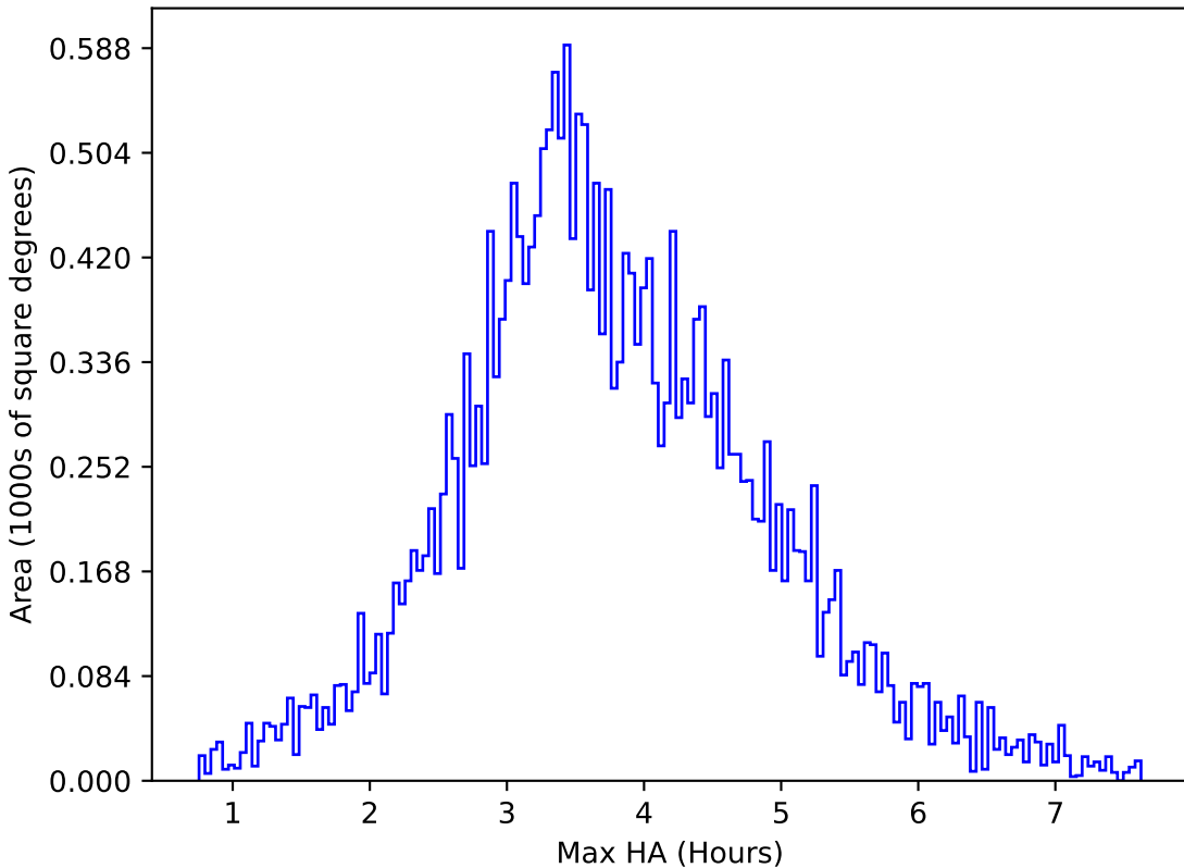
weather_cloudso10v3.4_10yrs All sky g band: Max HA
