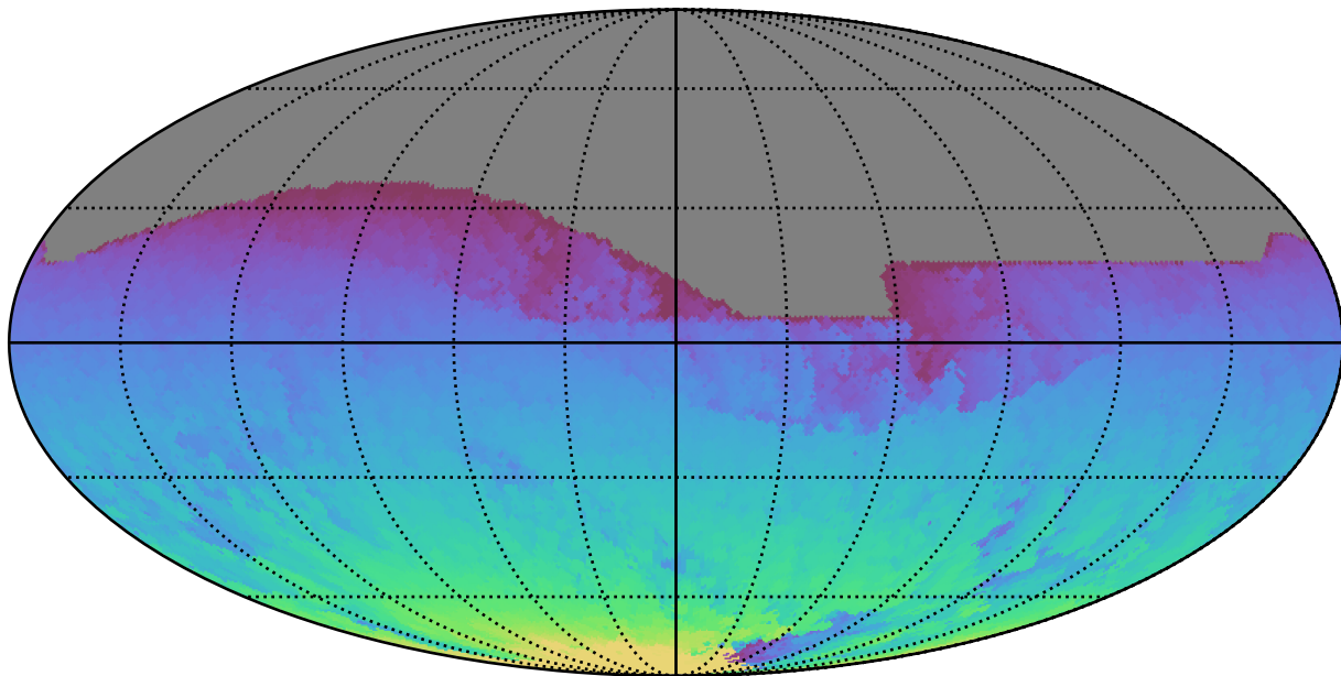
weather_cloudso10v3.4_10yrs All sky all bands: Max HA
