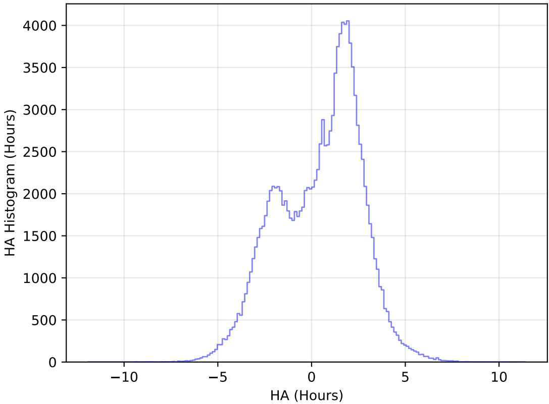
weather_cloudso10v3.4_10yrs WFD u band: HA Histogram
