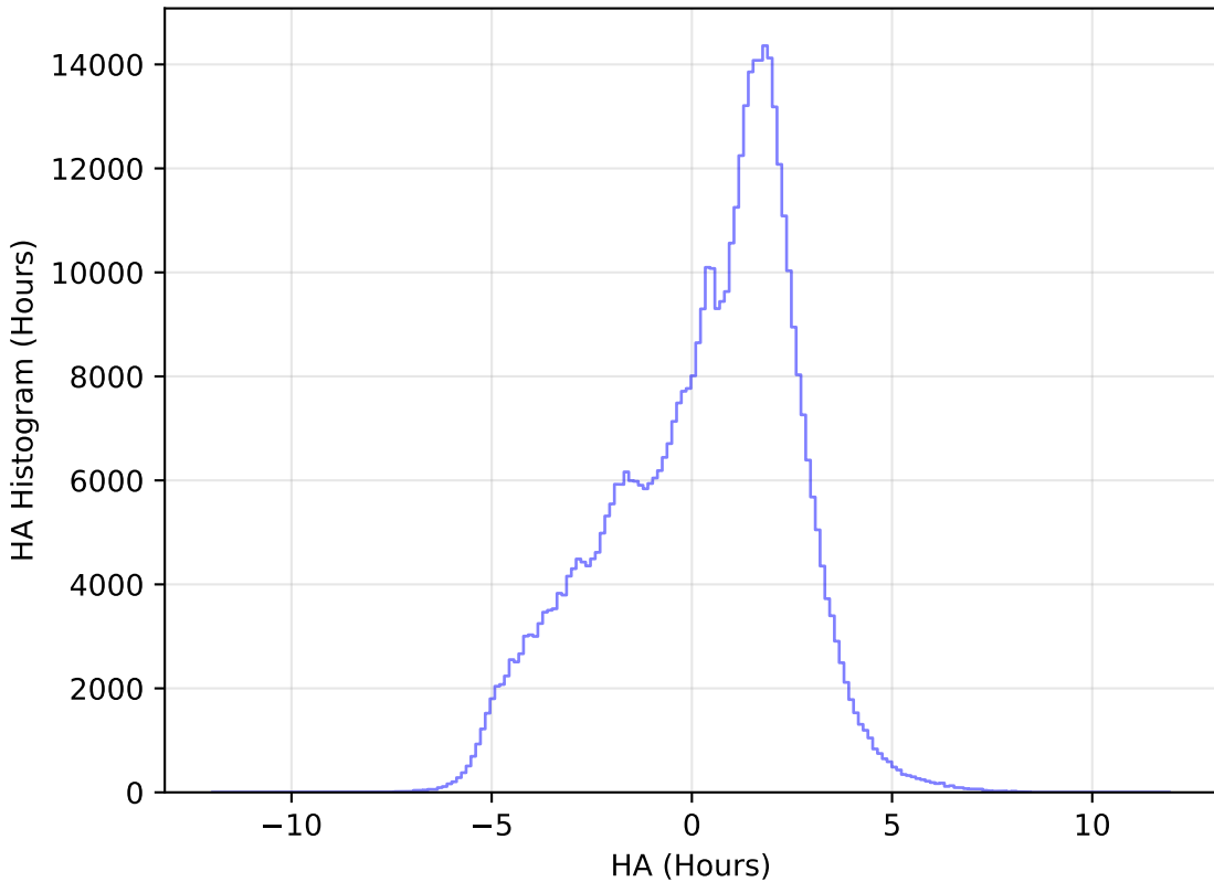
weather_cloudso10v3.4_10yrs WFD r band: HA Histogram
