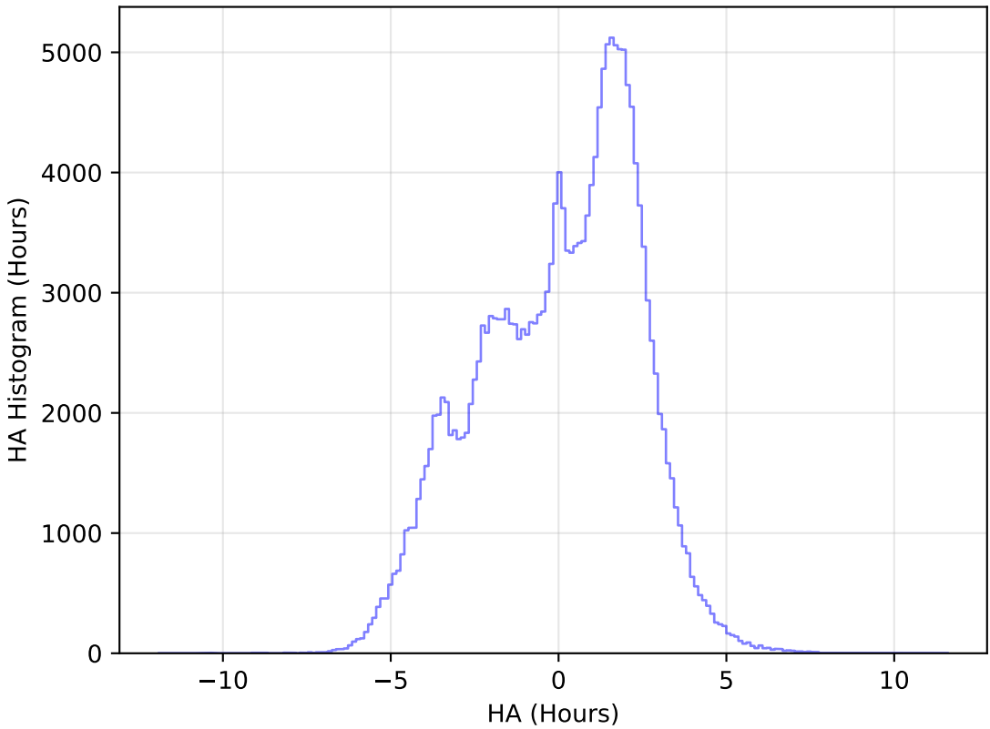
weather_cloudso10v3.4_10yrs WFD g band: HA Histogram
