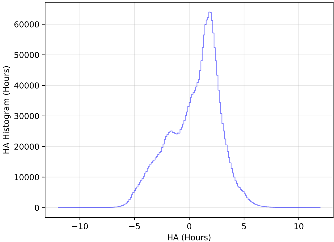
weather_cloudso10v3.4_10yrs WFD all bands: HA Histogram
