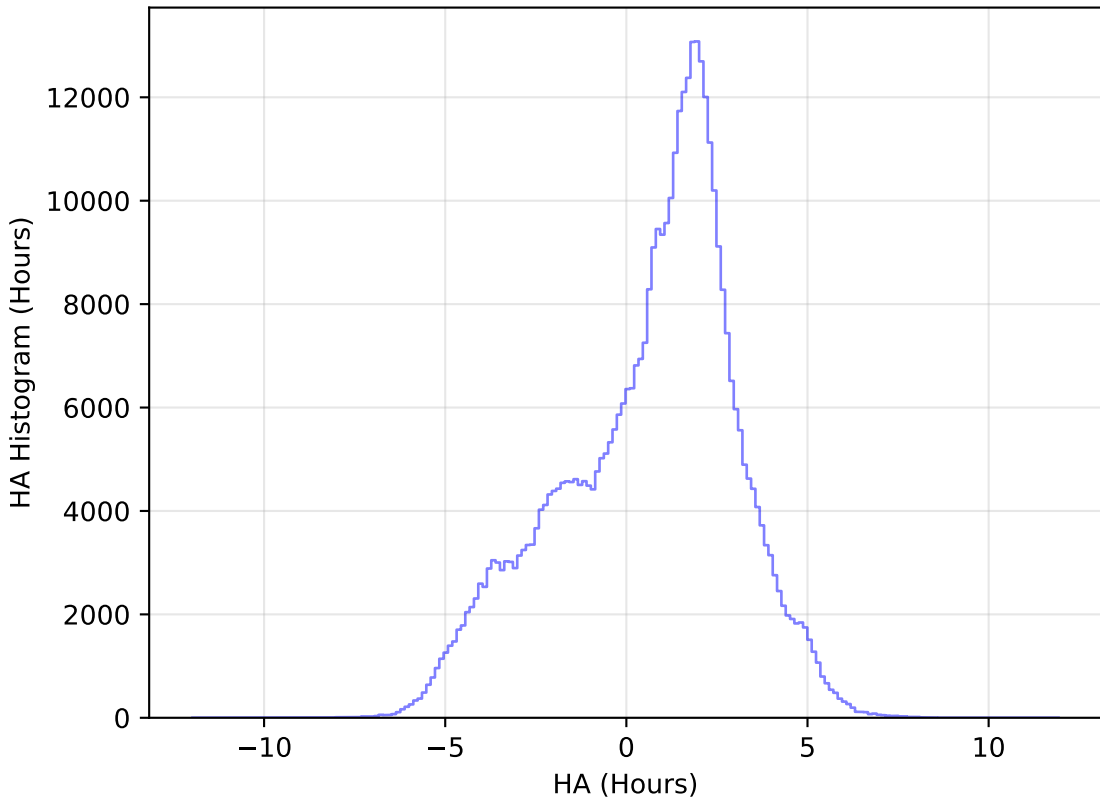
weather_cloudso10v3.4_10yrs All sky z band: HA Histogram
