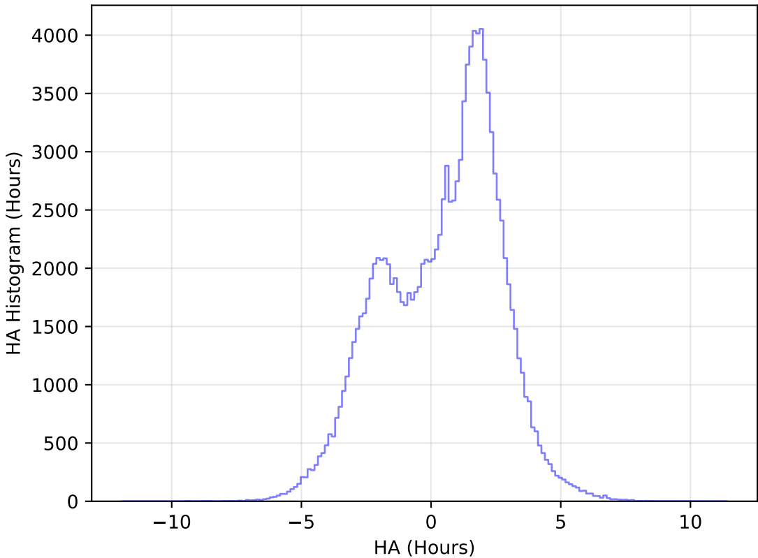
weather_cloudso10v3.4_10yrs All sky u band: HA Histogram
