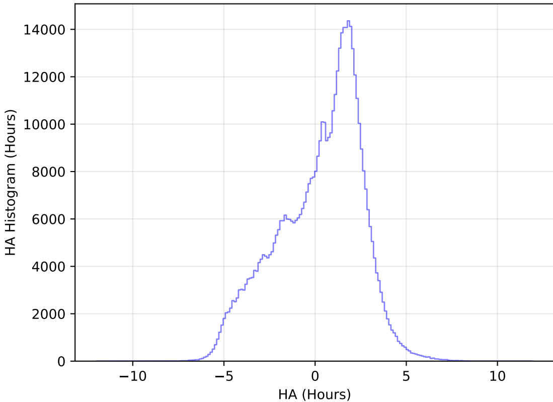
weather_cloudso10v3.4_10yrs All sky r band: HA Histogram
