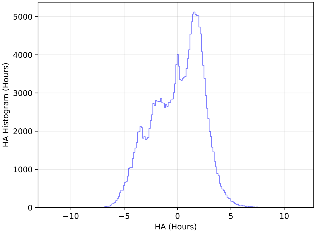
weather_cloudso10v3.4_10yrs All sky g band: HA Histogram
