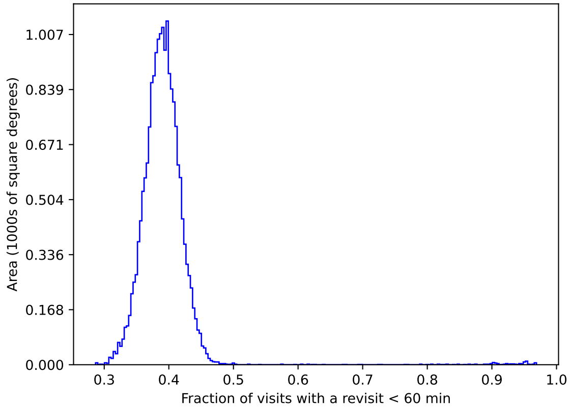
weather_cloudso10v3.4_10yrs gri WFD: Fraction of visits with a revisit < 60 min
