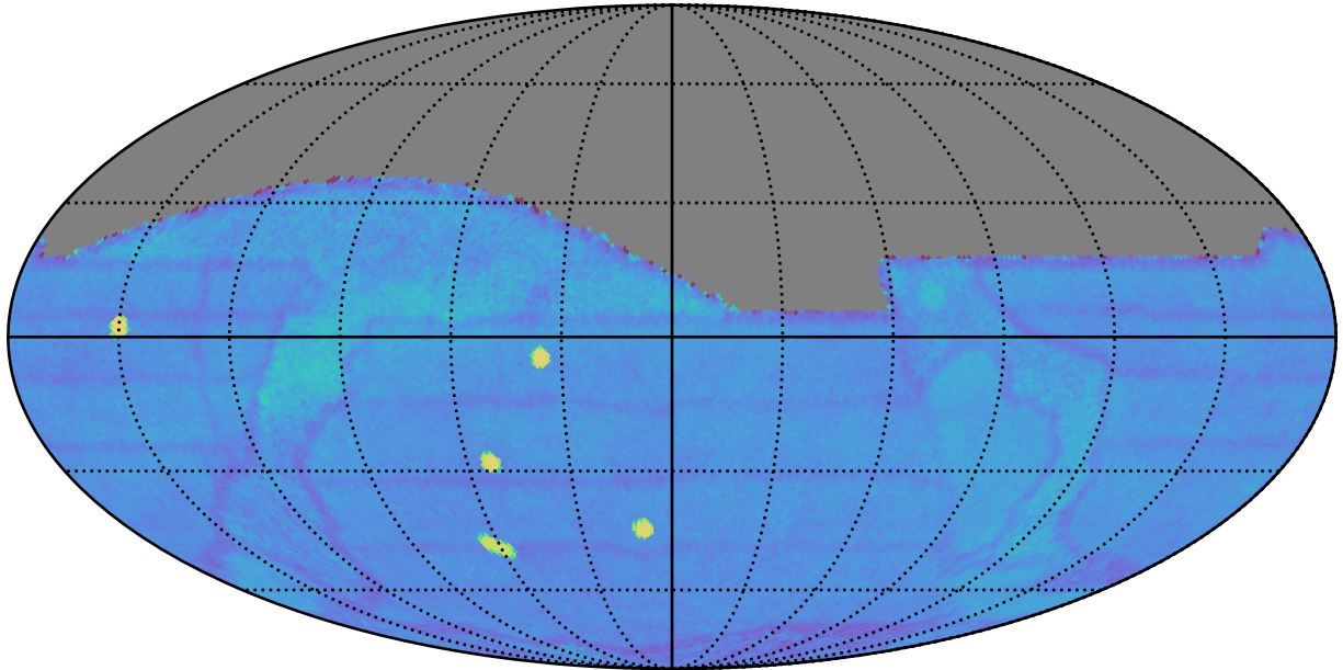
weather_cloudso10v3.4_10yrs gri All sky: Fraction of visits with a revisit < 60 min
