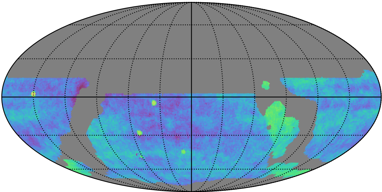
weather_cloudso10v3.4_10yrs gri WFD: Fraction of visits in pairs (20-90 min)
