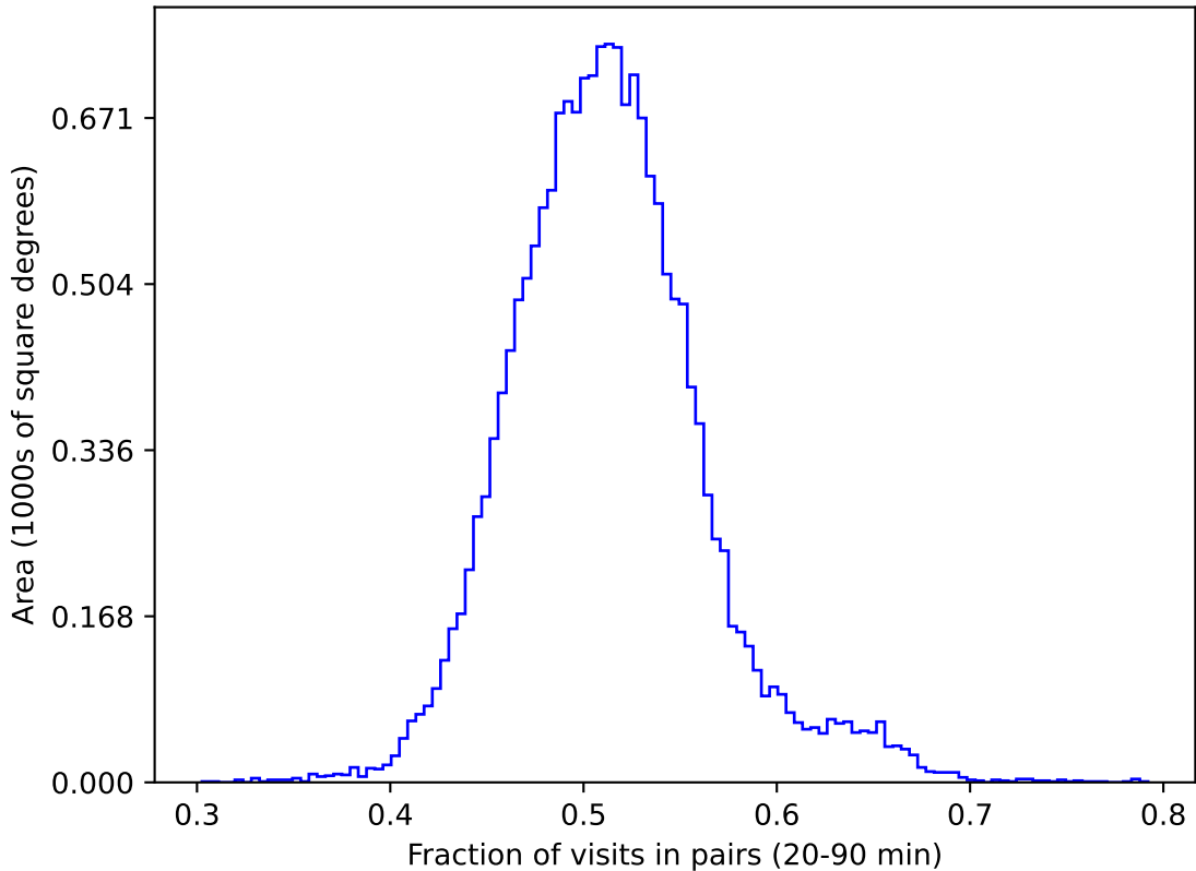
weather_cloudso10v3.4_10yrs gri WFD: Fraction of visits in pairs (20-90 min)
