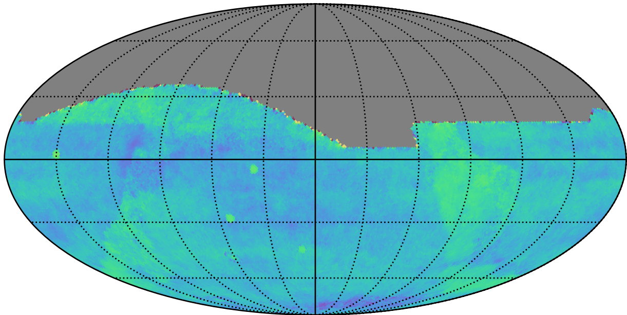
weather_cloudso10v3.4_10yrs gri All sky: Fraction of visits in pairs (20-90 min)
