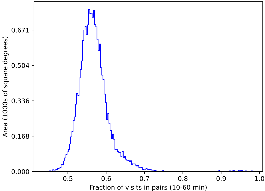
weather_cloudso10v3.4_10yrs gri WFD: Fraction of visits in pairs (10-60 min)
