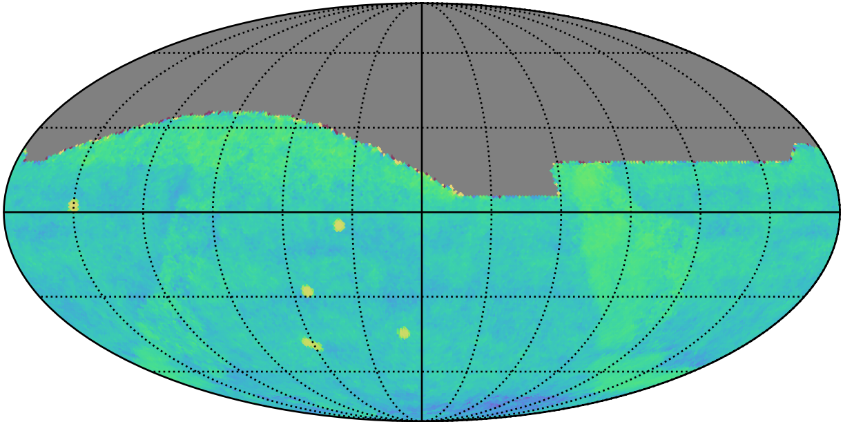
weather_cloudso10v3.4_10yrs gri All sky: Fraction of visits in pairs (10-60 min)
