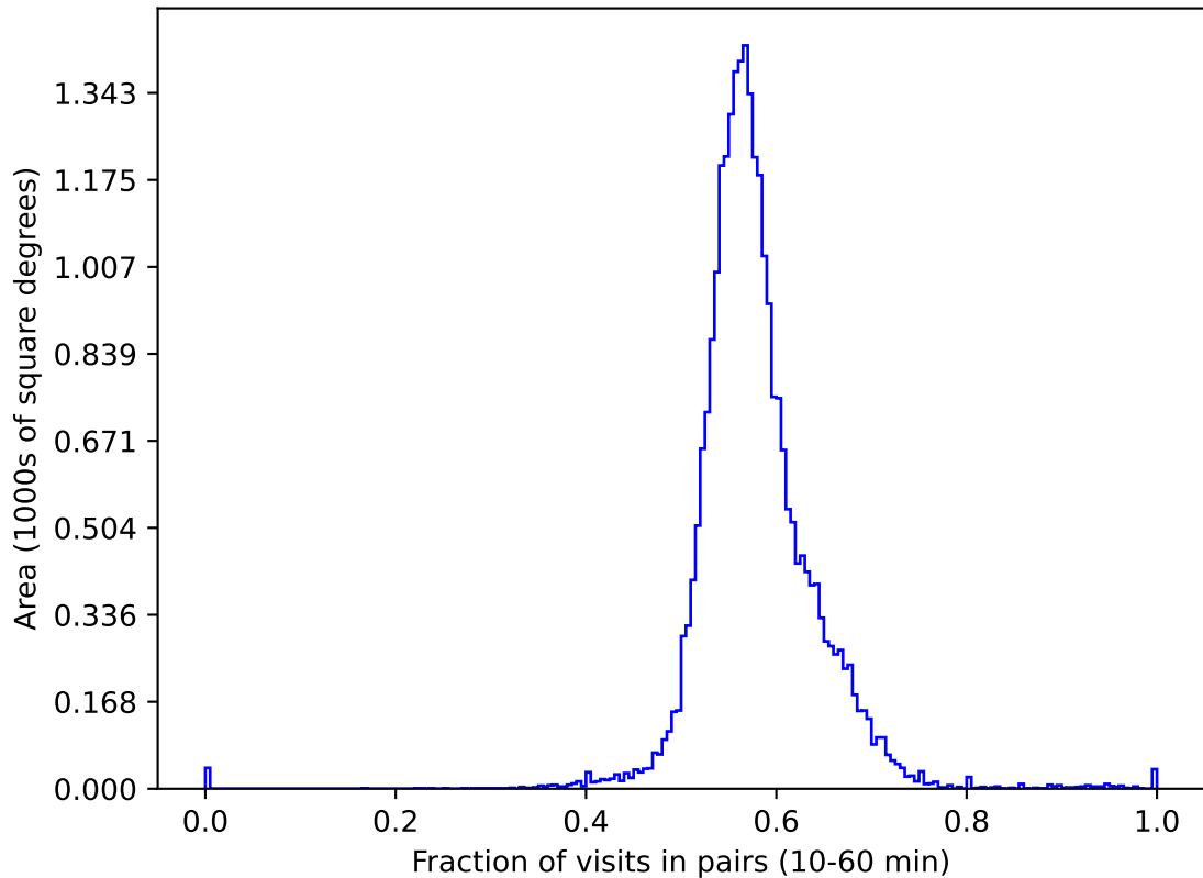
weather_cloudso10v3.4_10yrs gri All sky: Fraction of visits in pairs (10-60 min)
