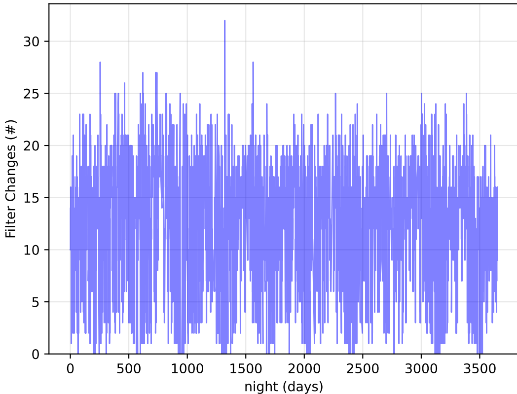
weather_cloudso10v3.4_10yrs Per Night: Filter Changes
