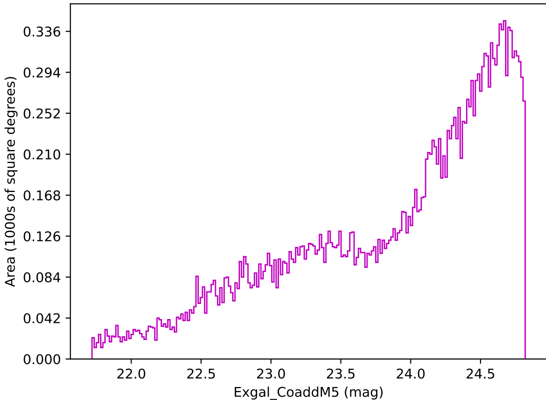
weather_cloudso10v3.4_10yrs Yr 3-4 z band: Exgal_CoaddM5
