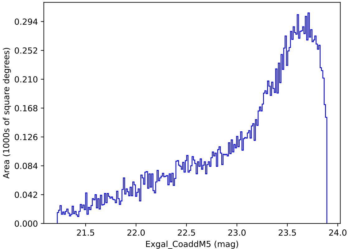
weather_cloudso10v3.4_10yrs Yr 3-4 y band: Exgal_CoaddM5
