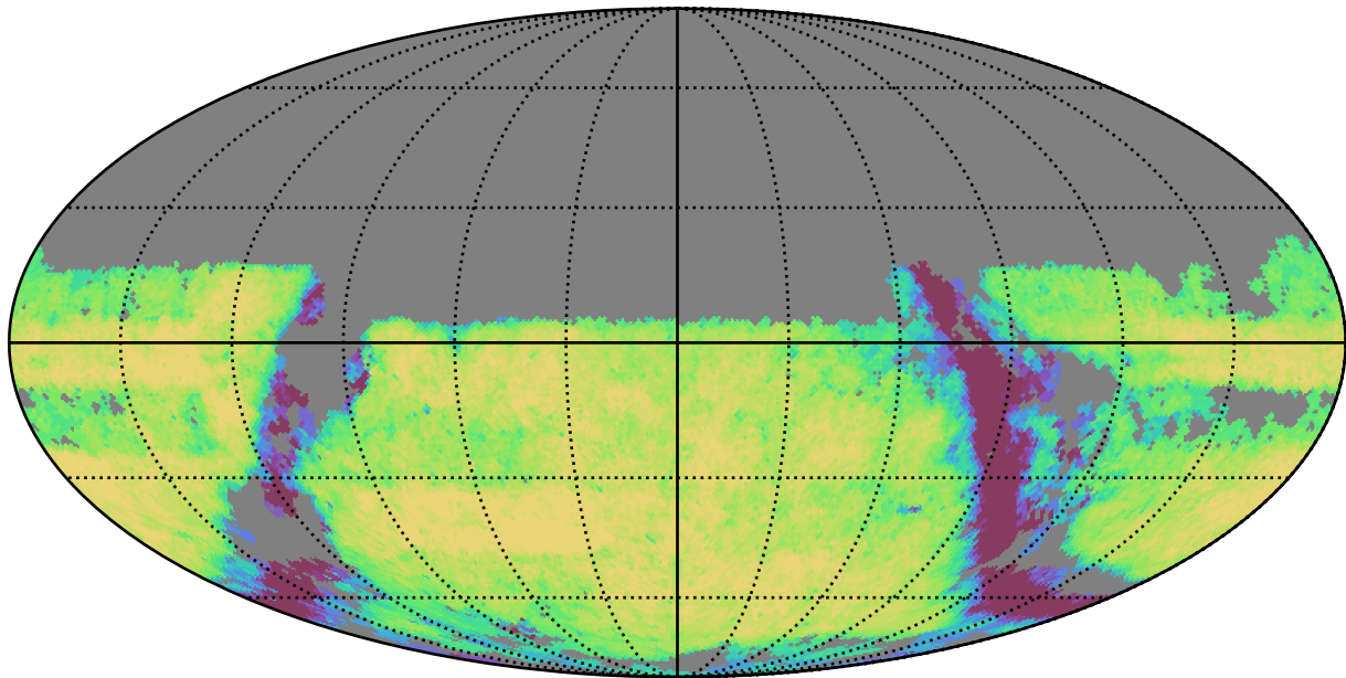
weather_cloudso10v3.4_10yrs Yr 3-4 u band: Exgal_CoaddM5
