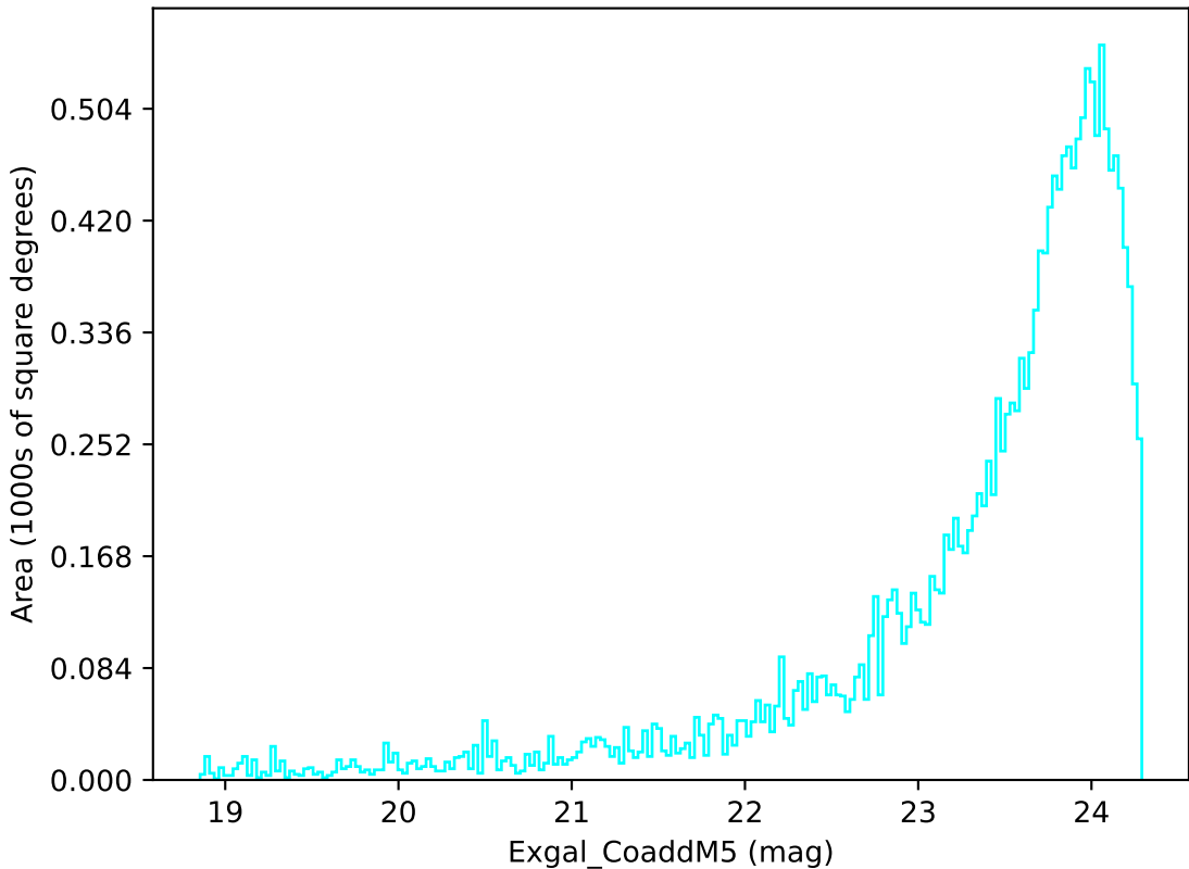
weather_cloudso10v3.4_10yrs Yr 3-4 u band: Exgal_CoaddM5
