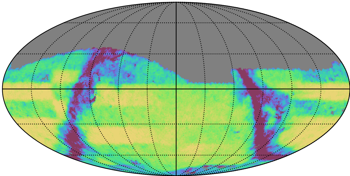
weather_cloudso10v3.4_10yrs Yr 3-4 r band: Exgal_CoaddM5
