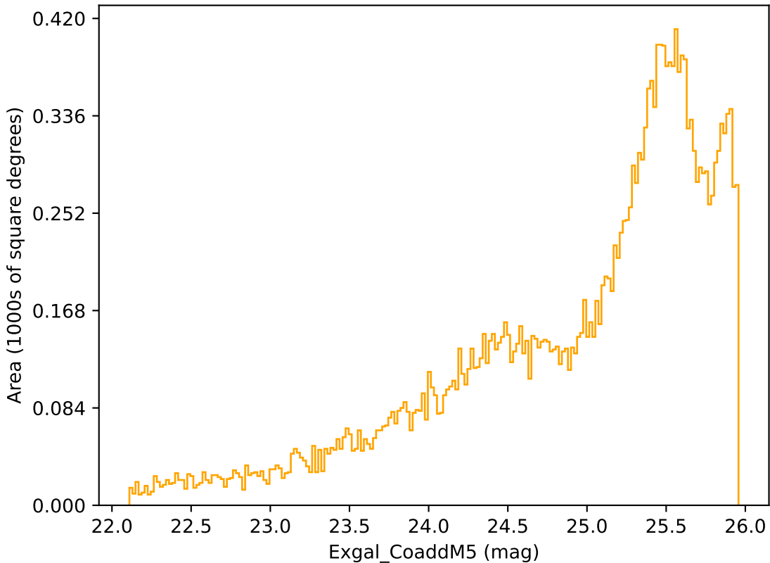
weather_cloudso10v3.4_10yrs Yr 3-4 r band: Exgal_CoaddM5
