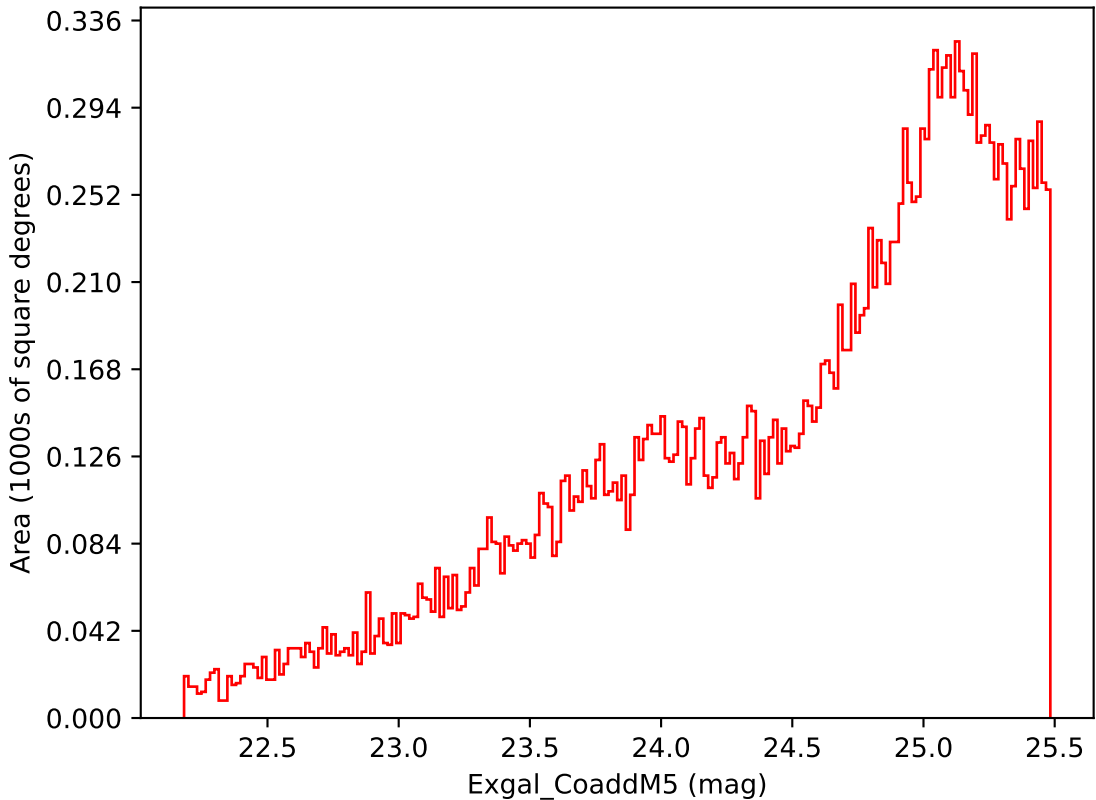
weather_cloudso10v3.4_10yrs Yr 3-4 i band: Exgal_CoaddM5
