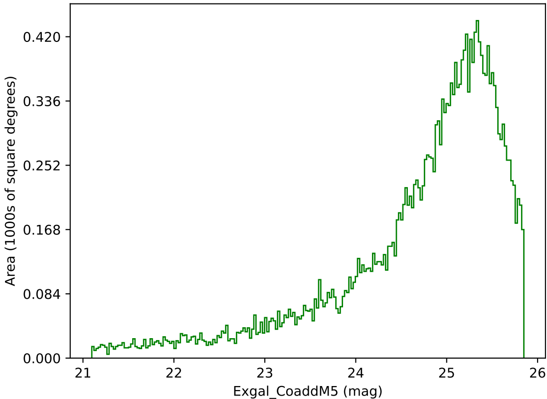
weather_cloudso10v3.4_10yrs Yr 3-4 g band: Exgal_CoaddM5
