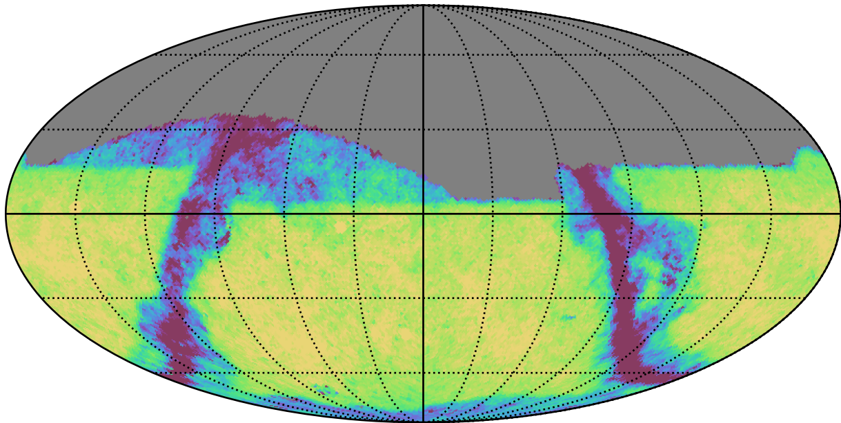
weather_cloudso10v3.4_10yrs Yr 1 z band: Exgal_CoaddM5
