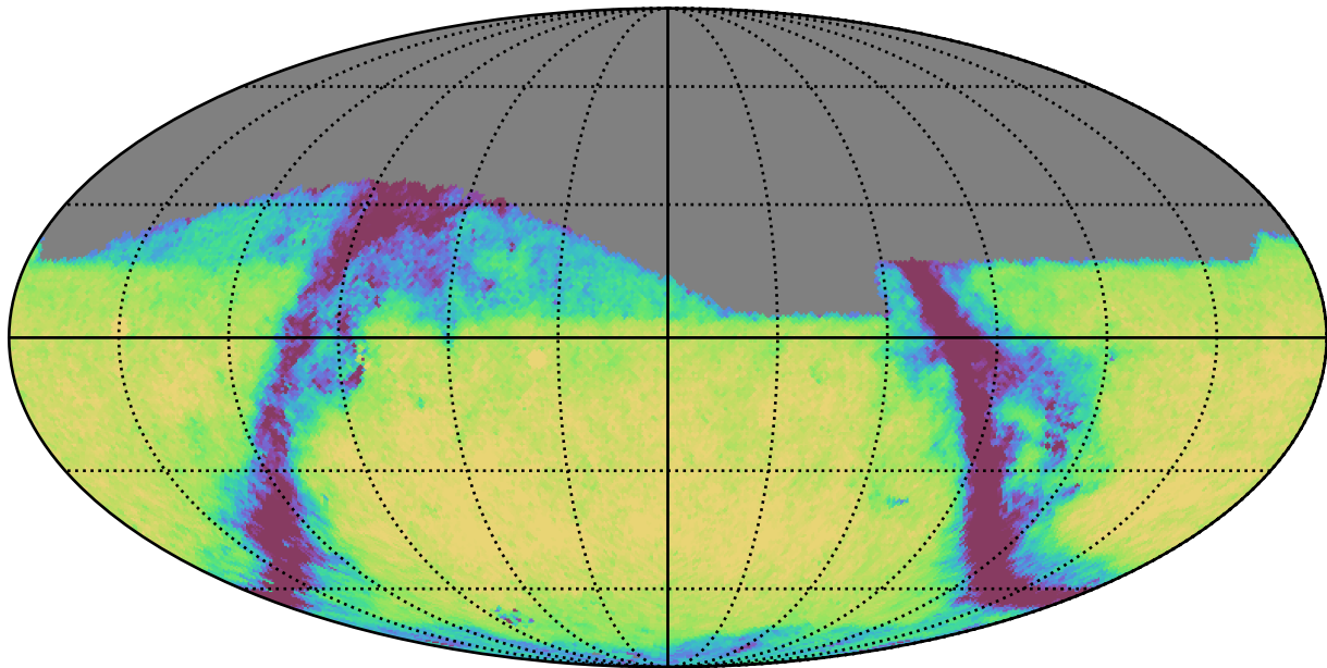
weather_cloudso10v3.4_10yrs Yr 1 r band: Exgal_CoaddM5
