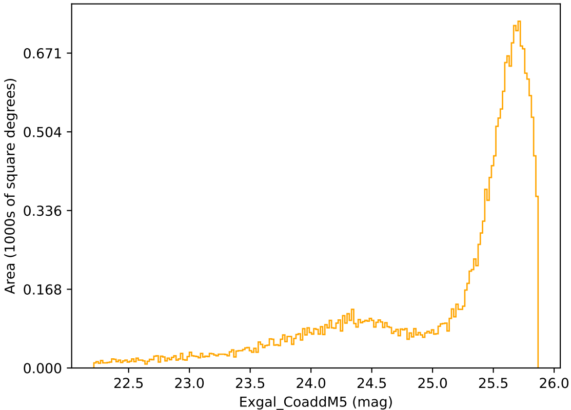
weather_cloudso10v3.4_10yrs Yr 1 r band: Exgal_CoaddM5
