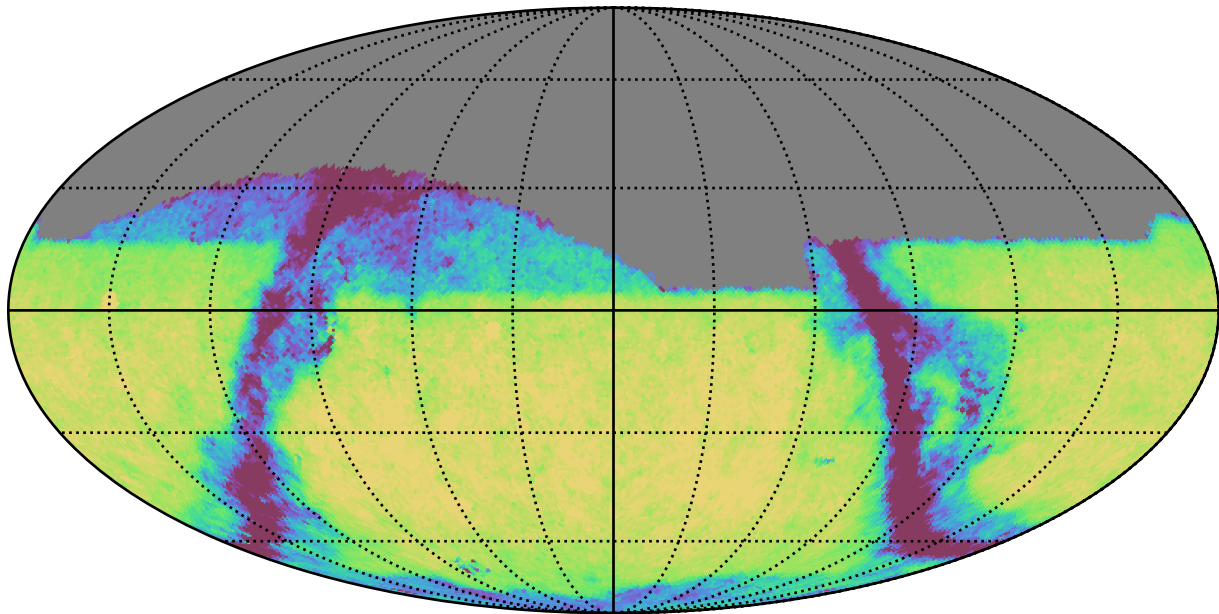
weather_cloudso10v3.4_10yrs Yr 1 i band: Exgal_CoaddM5
