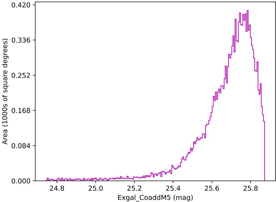
weather_cloudso10v3.4_10yrs WFD z band: Exgal_CoaddM5
