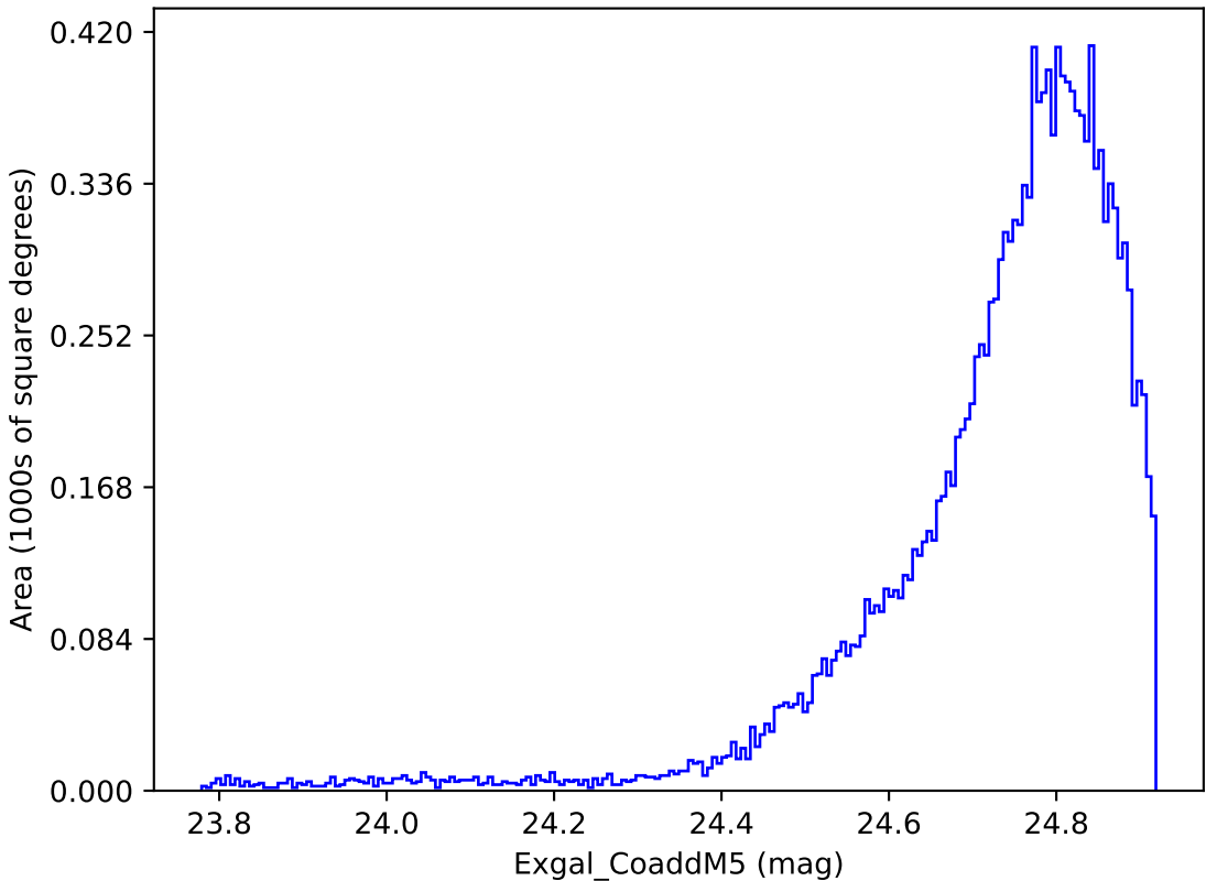
weather_cloudso10v3.4_10yrs WFD y band: Exgal_CoaddM5
