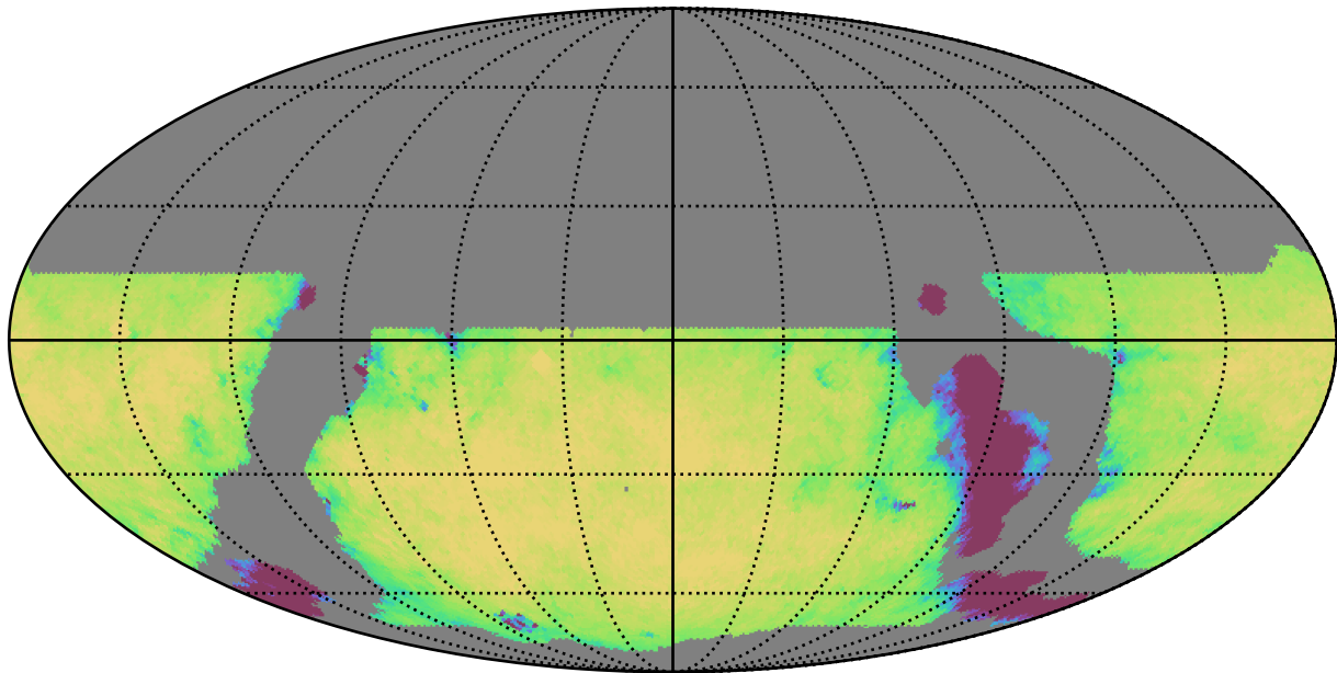
weather_cloudso10v3.4_10yrs WFD u band: Exgal_CoaddM5
