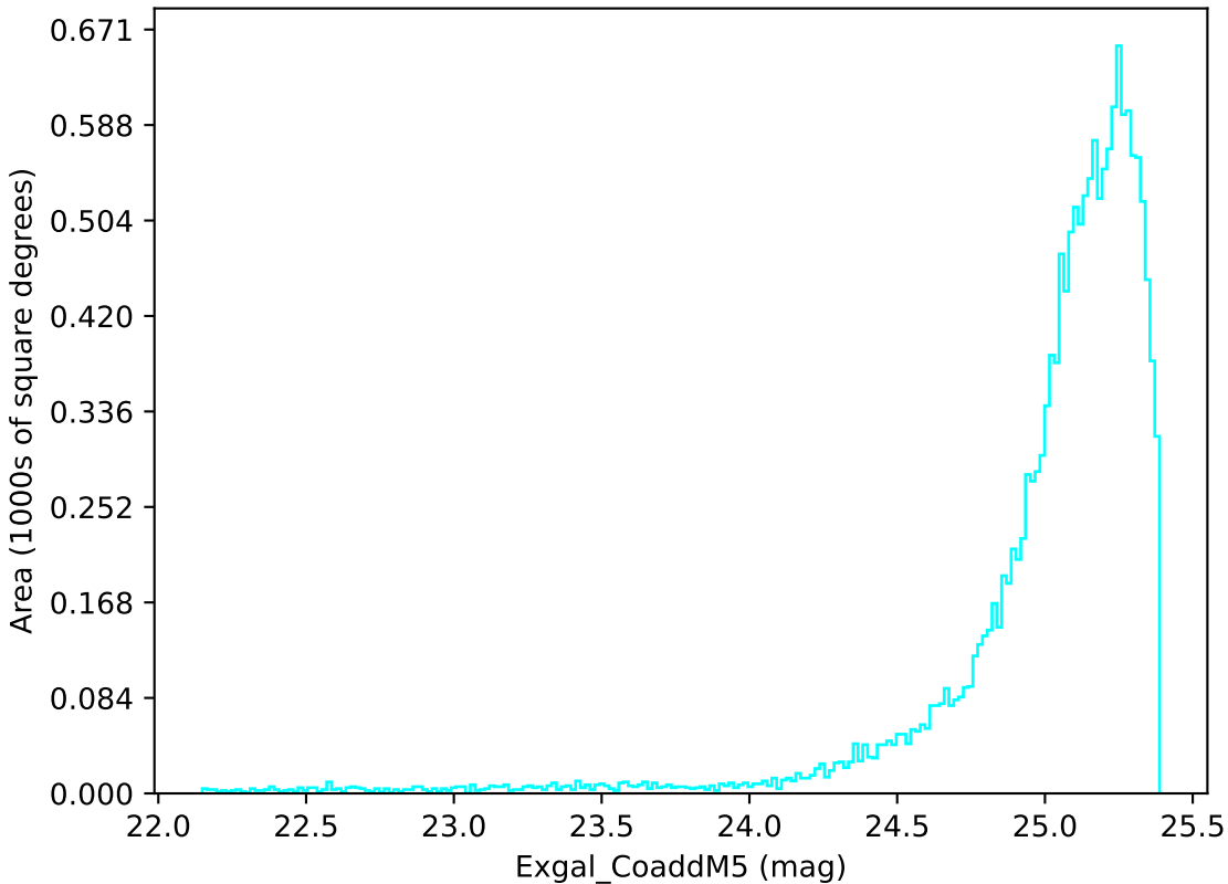
weather_cloudso10v3.4_10yrs WFD u band: Exgal_CoaddM5
