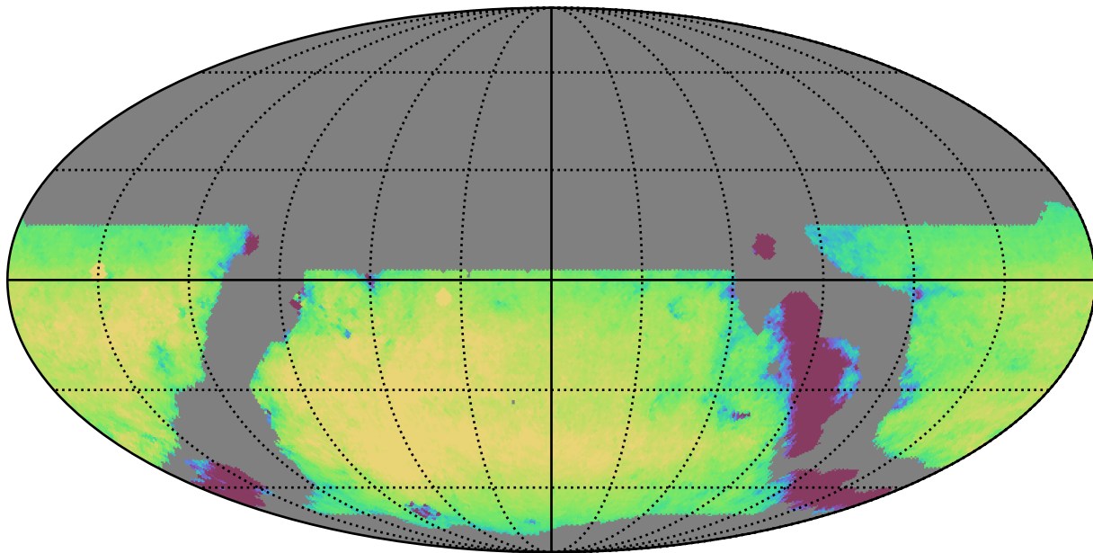
weather_cloudso10v3.4_10yrs WFD r band: Exgal_CoaddM5
