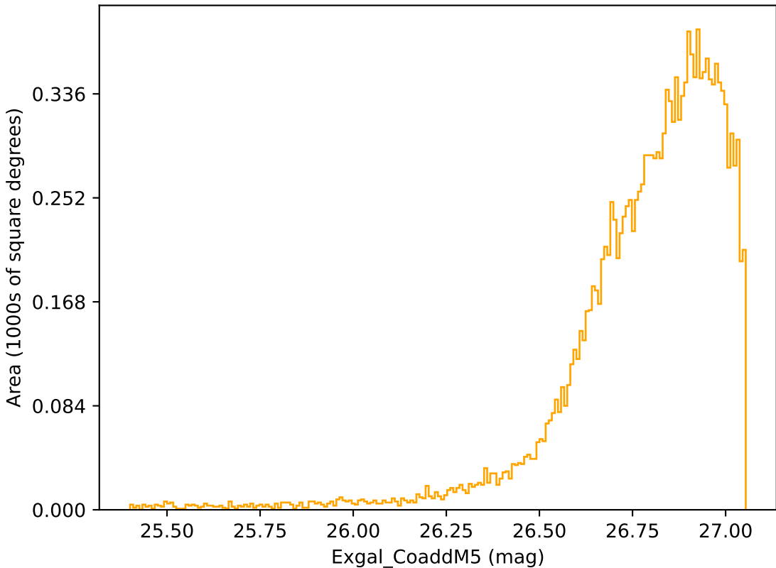
weather_cloudso10v3.4_10yrs WFD r band: Exgal_CoaddM5
