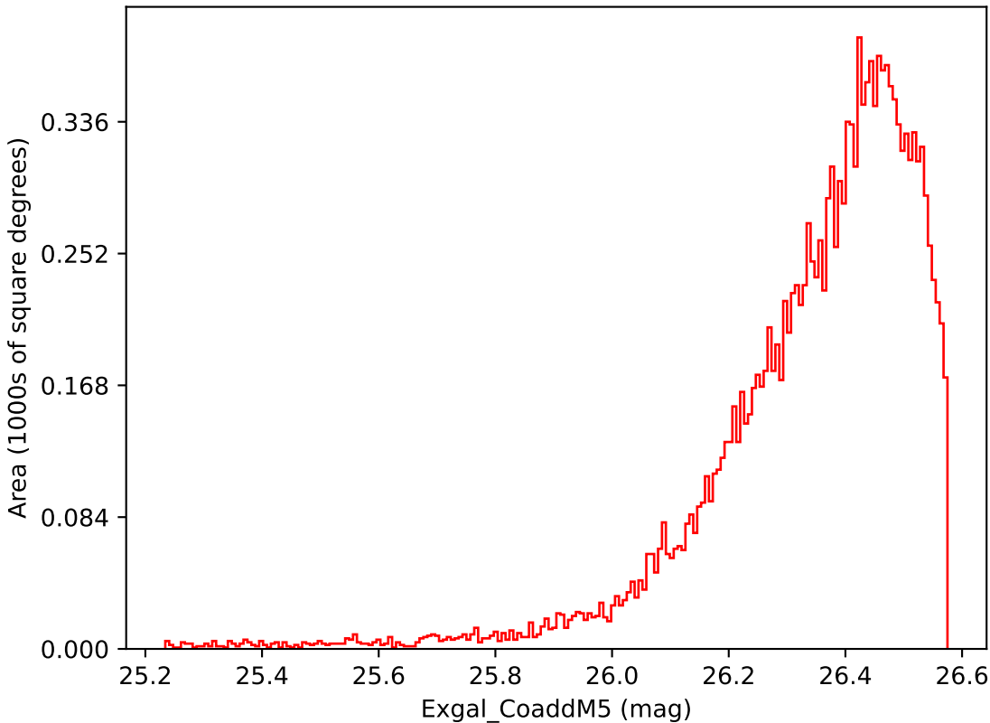
weather_cloudso10v3.4_10yrs WFD i band: Exgal_CoaddM5
