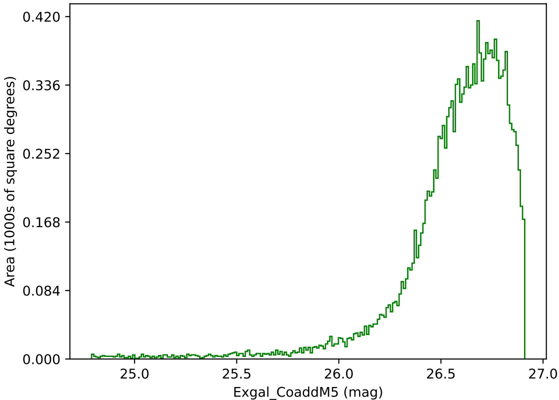
weather_cloudso10v3.4_10yrs WFD g band: Exgal_CoaddM5
