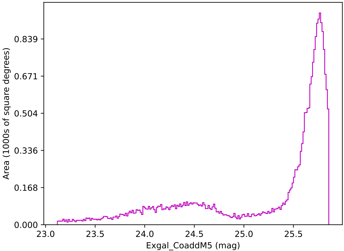
weather_cloudso10v3.4_10yrs All sky z band: Exgal_CoaddM5
