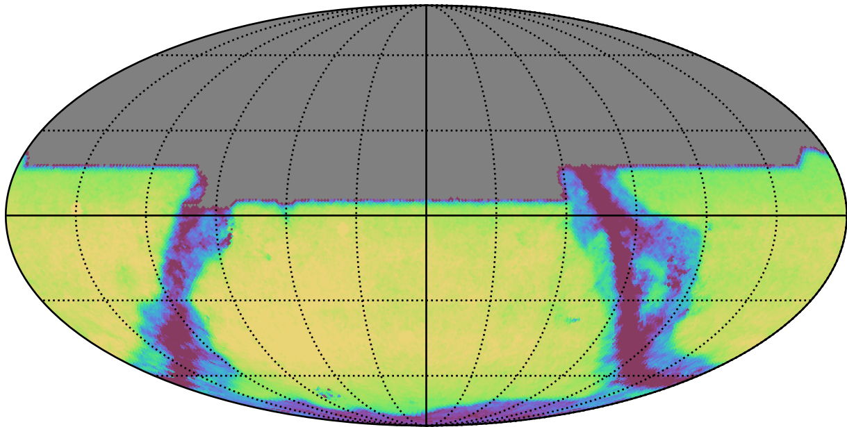
weather_cloudso10v3.4_10yrs All sky y band: Exgal_CoaddM5
