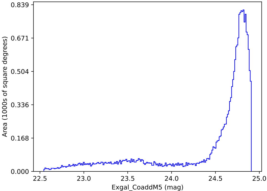
weather_cloudso10v3.4_10yrs All sky y band: Exgal_CoaddM5
