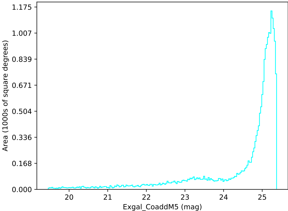
weather_cloudso10v3.4_10yrs All sky u band: Exgal_CoaddM5
