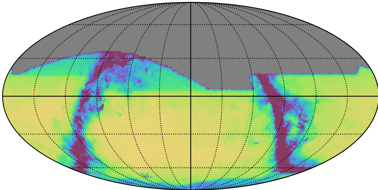
weather_cloudso10v3.4_10yrs All sky r band: Exgal_CoaddM5
