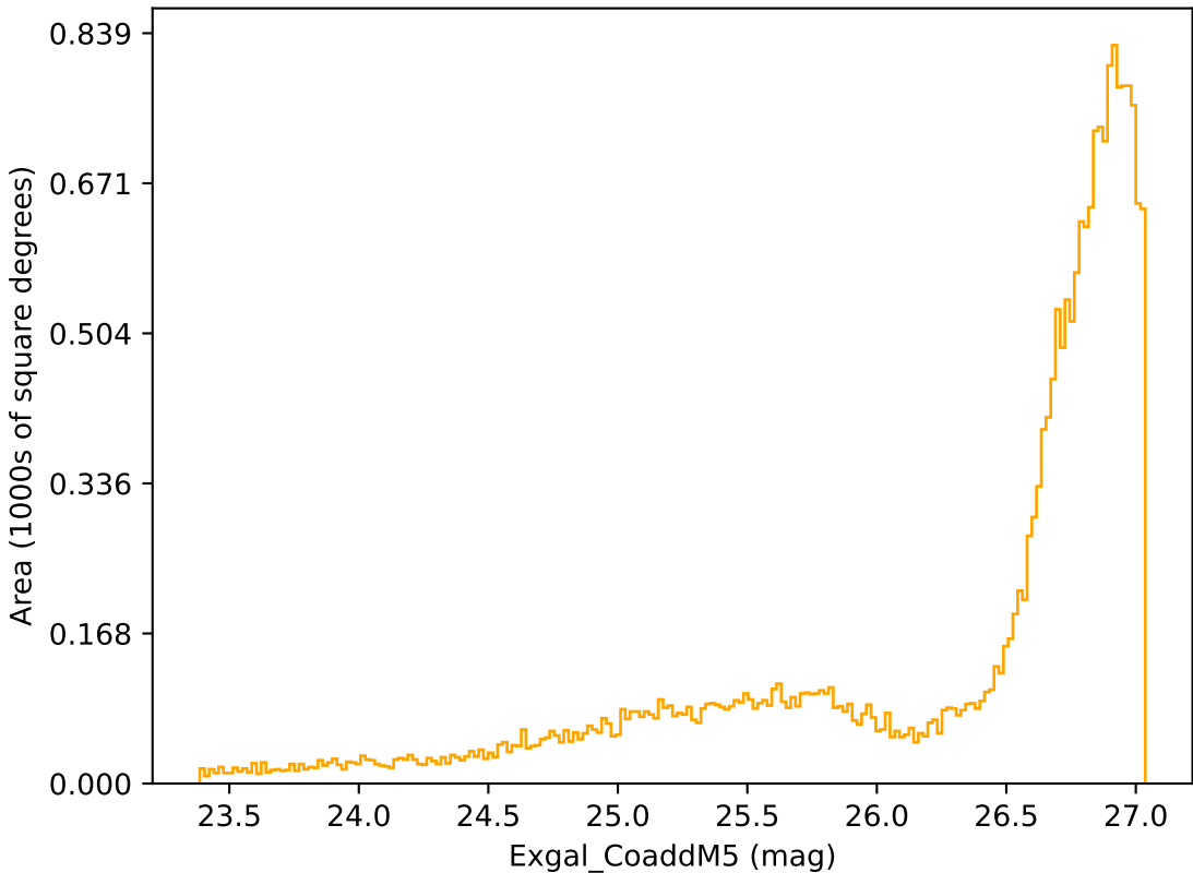
weather_cloudso10v3.4_10yrs All sky r band: Exgal_CoaddM5
