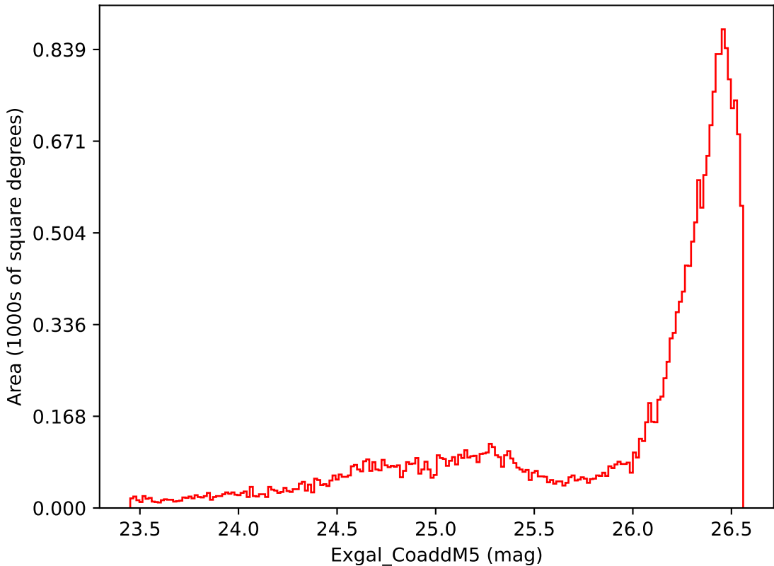
weather_cloudso10v3.4_10yrs All sky i band: Exgal_CoaddM5
